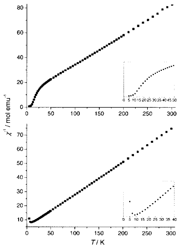
Fig. 7 The inverse molar magnetic susceptibility of polycrystalline \text{Mn}_3(\text{O}_3\text{PCH}_2\text{CH}_2\text{COO})_2 (bottom) and \text{Mn}_3(\text{O}_3\text{PCH}_2\text{COO})_2 (top) plotted as a function of the temperature (5–300 K).
